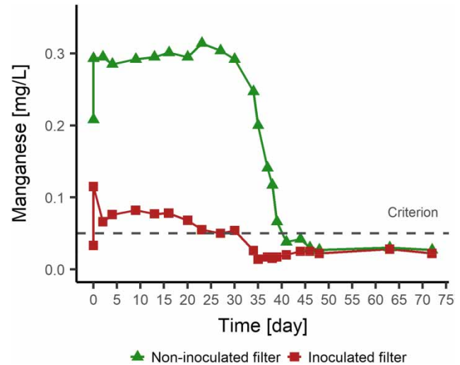
Figure 2 | Manganese concentration over time at the outlet of the pilot biofilters with and without inoculation.
